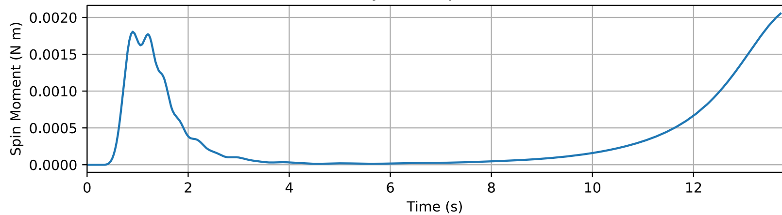
Aerodynamic Spin Moment
