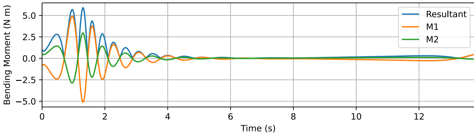
Aerodynamic Bending Resultant Moment
